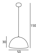
SQ-3650MP White 1x60W E27 230V
