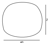
C0237-05M 5x40W G9 230V
