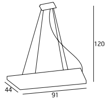
P0013 2x40W 2GX13 230V
