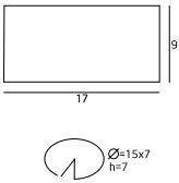
DK-02 WH 2x35W GU5.3 12V
