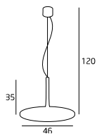
P0101 1x28W LED 230V 3000LM 1380LM
