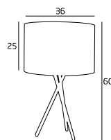
T0004 1x60W E27 230V
