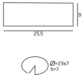
DK-03BK 3x35W GU5.3 12V
