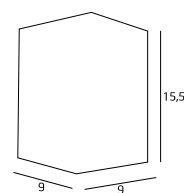
57-0721 1x40W G9 230V
