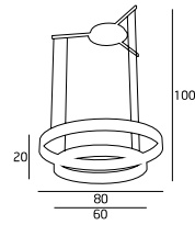
P0016 30W+22W LED 230V 3000K 3180LM
