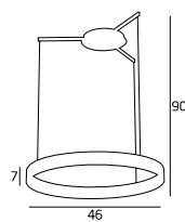
P0052 17,3W LED 230V 3000K 1020LM
