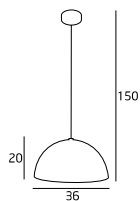
SQ-360MP White 1x60W E27 230V
