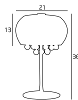
T0076-03D 3x40W G9 230V
