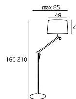
F0006 1x60W E27 230V
