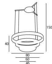
P0057 30W+22W+17,3 LED 230V 3000K 4200LM
