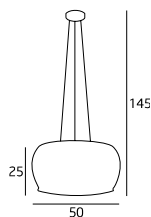
P0076-06X 6x40W G9 230V
