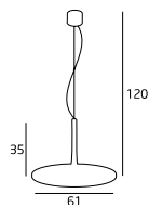
P0102 1x36W LED 230V 3000LM 2160LM
