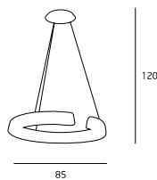
P0133 52W LED 230V 3600LM 3000K
