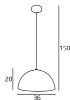
SQ-360MP Black 1x60W E27 230V
