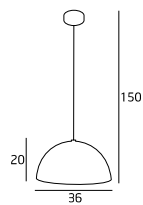
SQ-360MP Chrome 1x60W E27 230V
