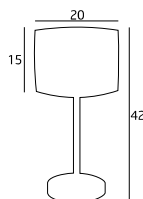
T0010 1x60W E27 230V
