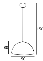
SQ-3650MP Chrome 1x60W E27 230V
