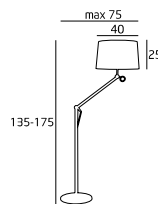
F0005 1x60W E27 230V
