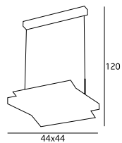
K2012 1x40W 2GX13 230V
