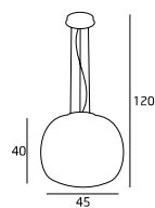
P0118 1x100W E27 230V
