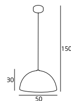
SQ-3650MP Black 1x60W E27 230V
