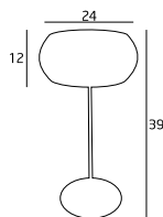
T0109-03A 3x40W G9 230V
