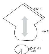
H0033 1x13W LED 230V 3000K 700LM
