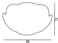
JX006-6 6x40W G9 230V
