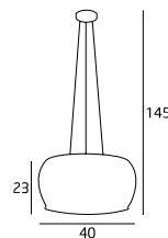
P0076-05L 5x40W G9 230V
