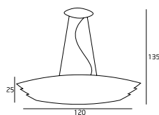
P0332-04M 4x60W E27 230V
