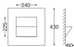
Druga metoda montowania / The second method of mounting
